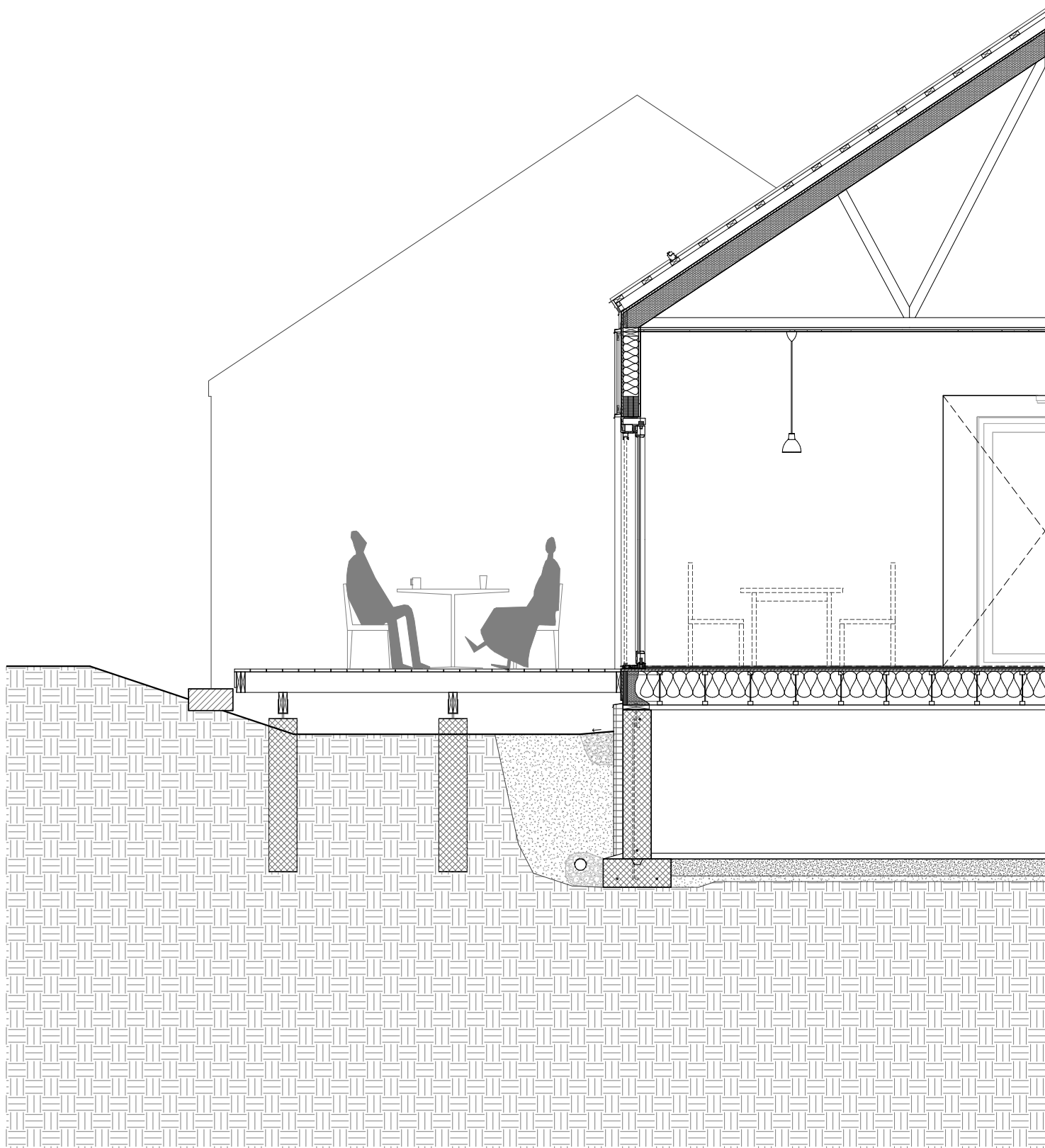
Building Section at Kitchen / Dining / Open air porch
