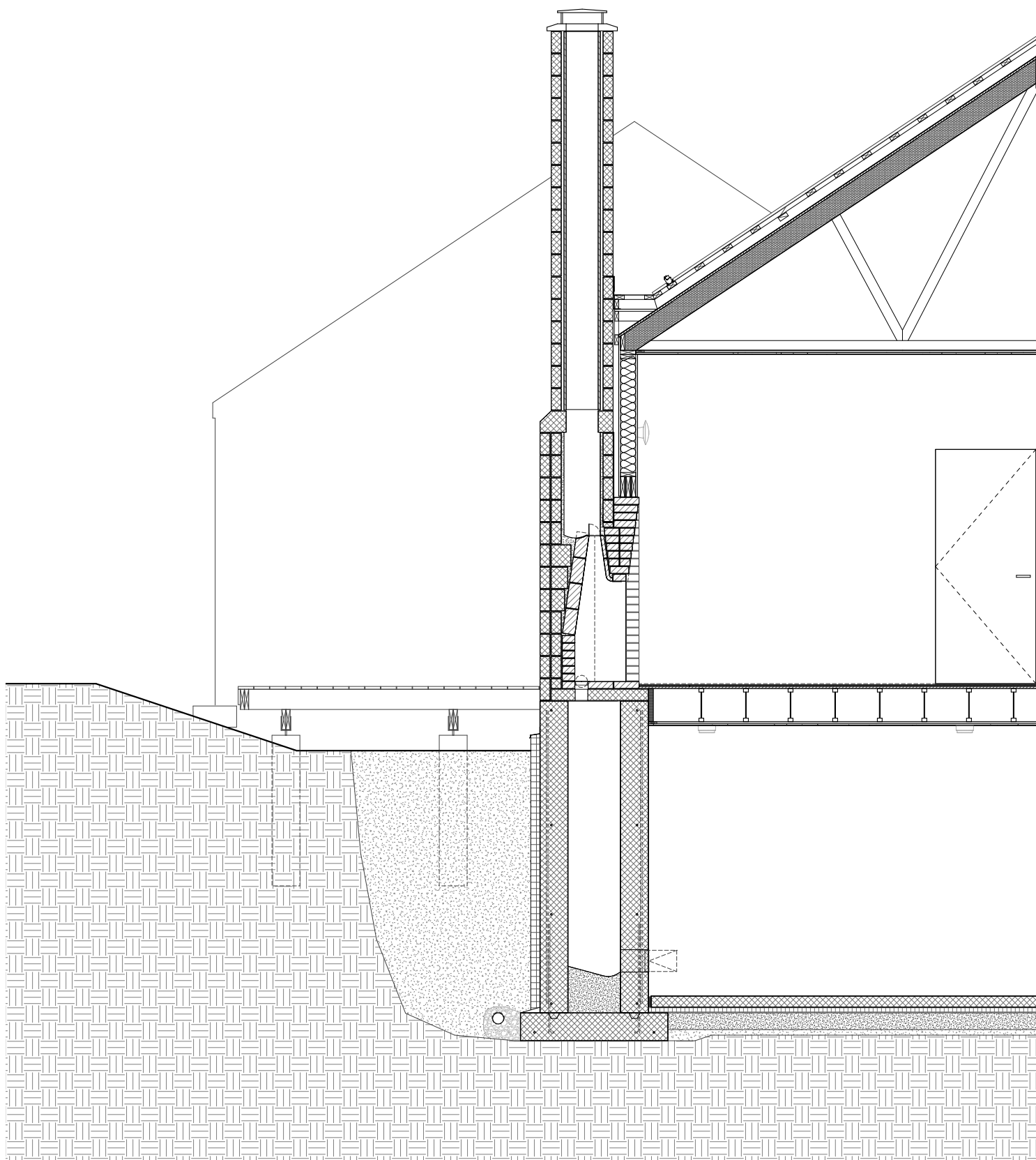
Building Section at Living Room
