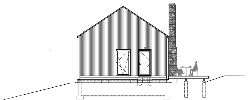
North Elevation
