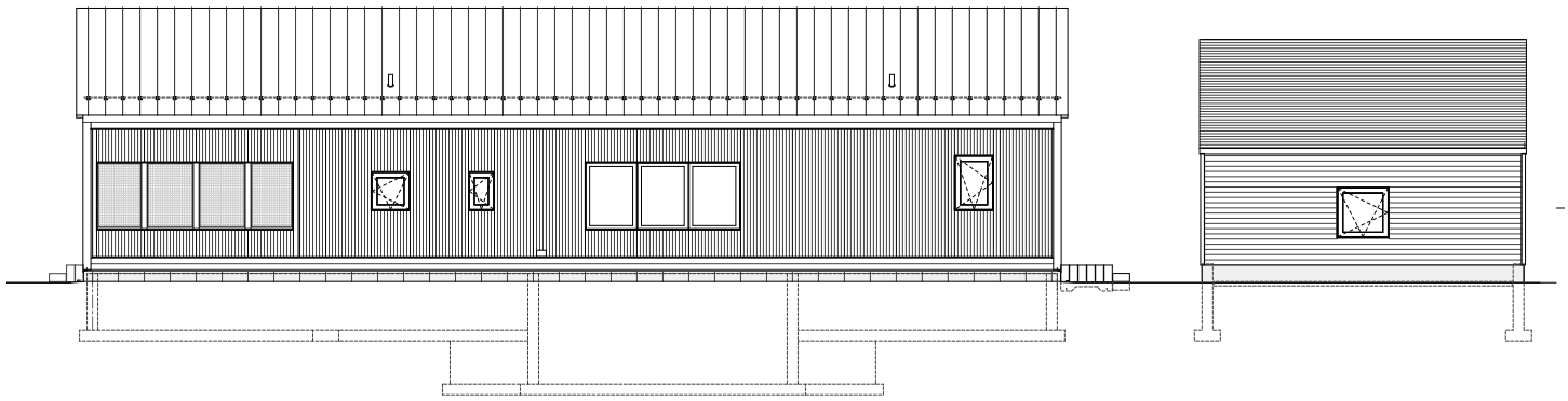
East Elevation
