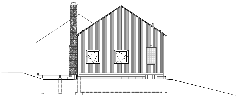
South Elevation
