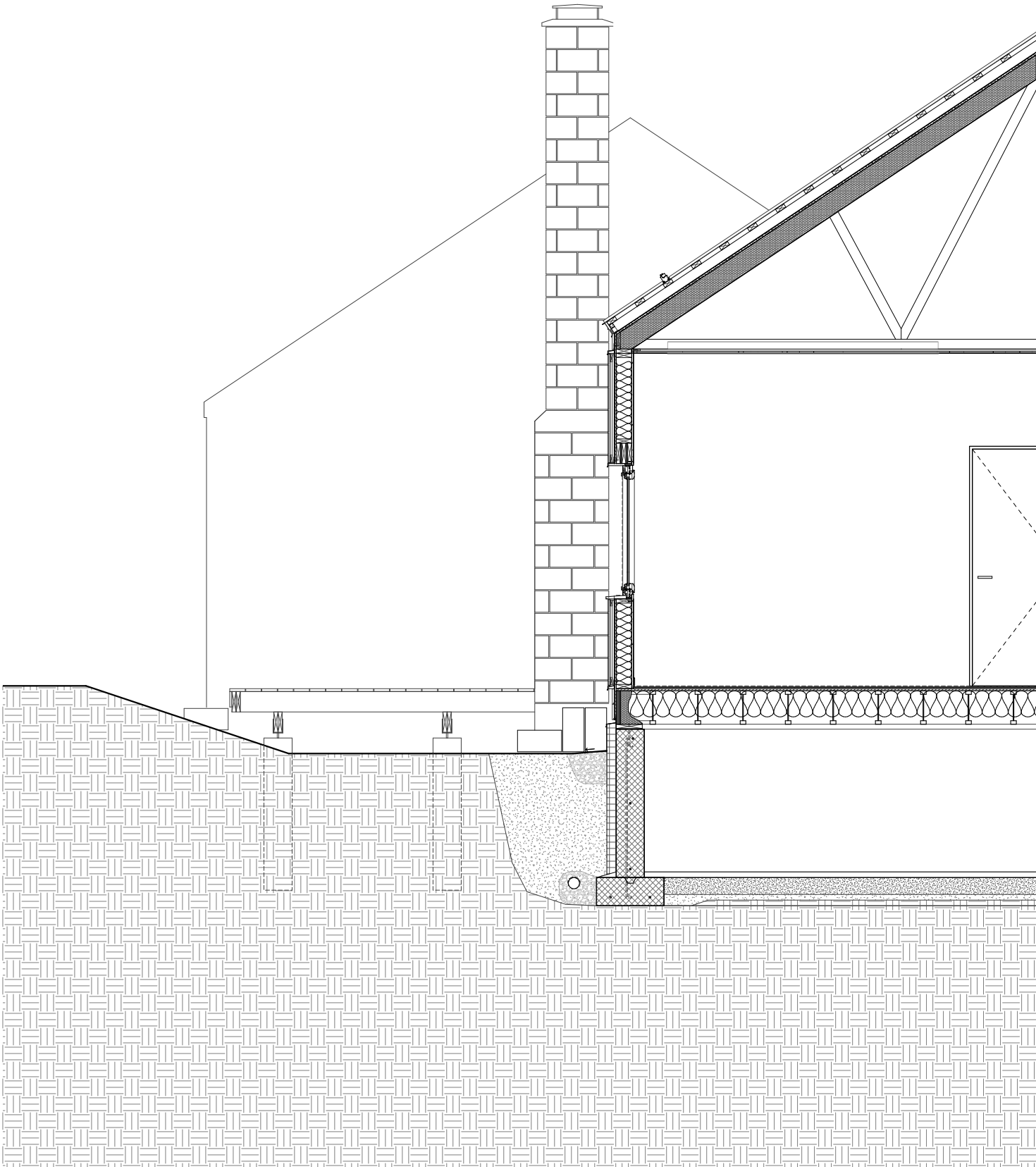
Building Section at Studio / Screened Porch
